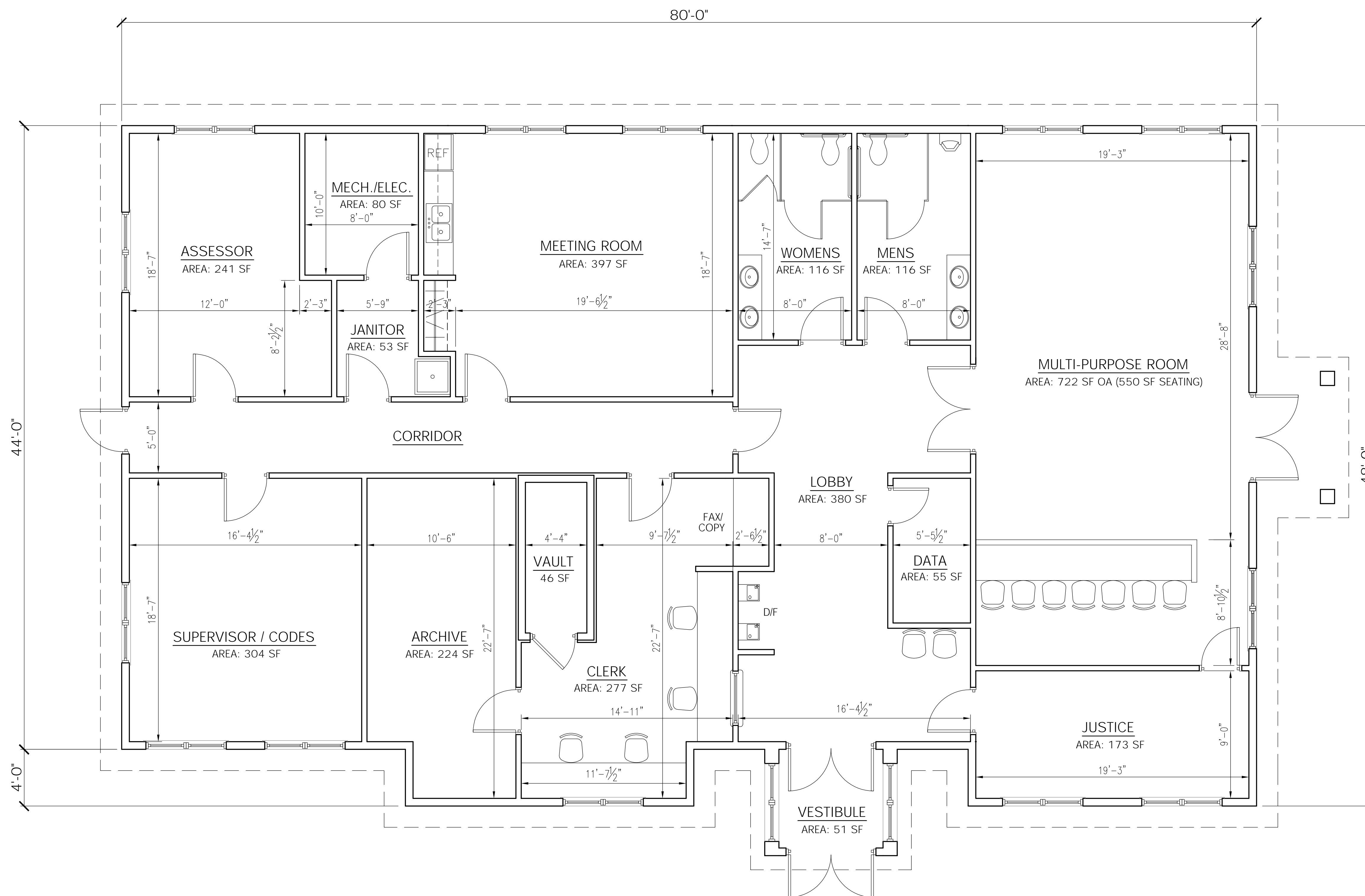
1 PROPOSED BUILDING FLOORPLAN A101 SCALE: 1/4"=1'-0" BUILDING AREA: 3,752 SQ. FT.
